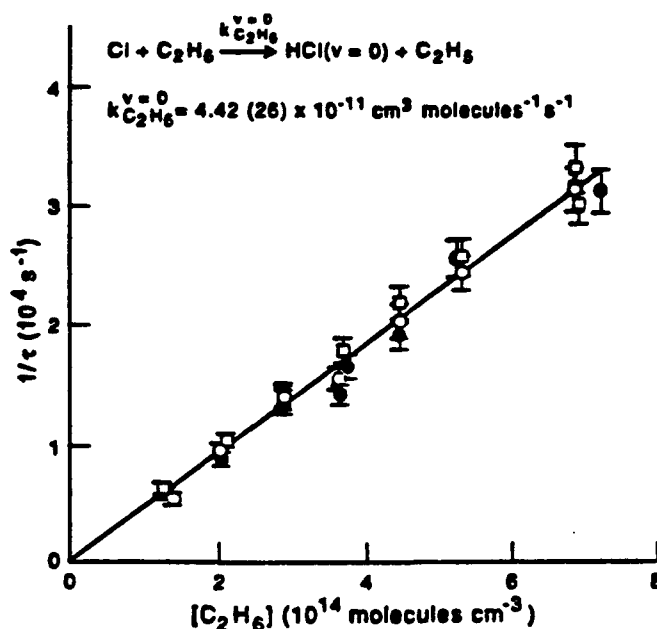
Fig. 9. Stern-Volmer plot for H atom abstraction of ethane by Cl radicals
